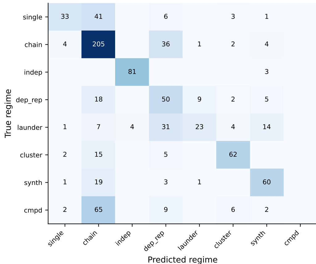
Form-aligned classifier
