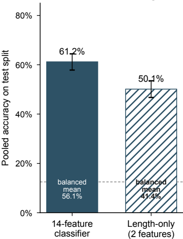
a Full features exceed length-only
