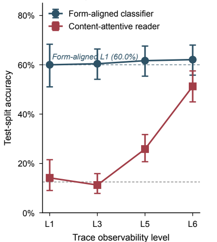
c Trace helps content-attentive readers
