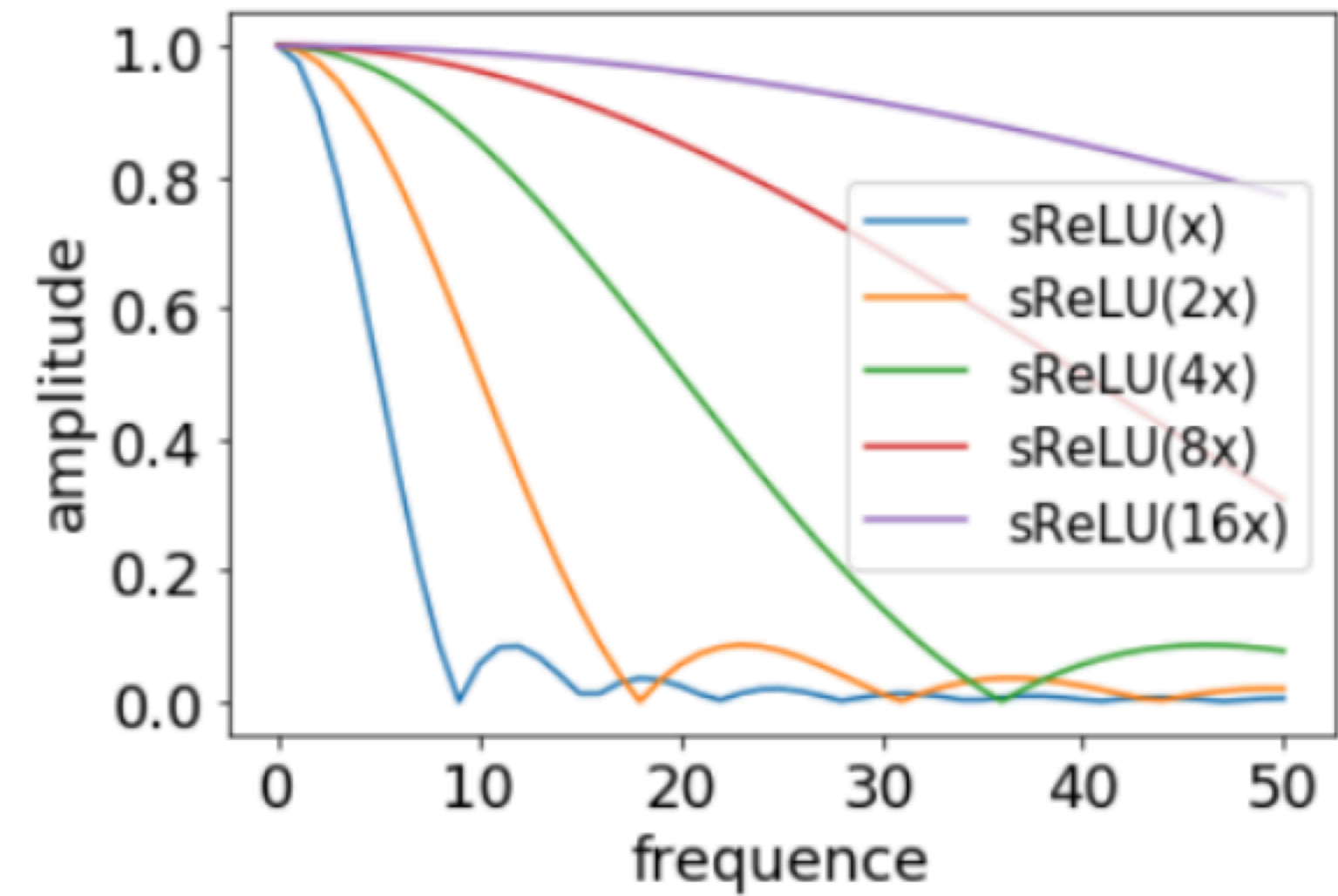
(a) sReLU
