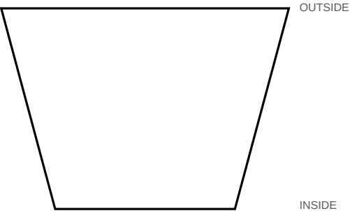
S1 · Ring 1 · make 12 12 segments · miter 15° each end Outside 2.144" · Inside 1.340" · Width 1.500" Stock thickness 0.750"
