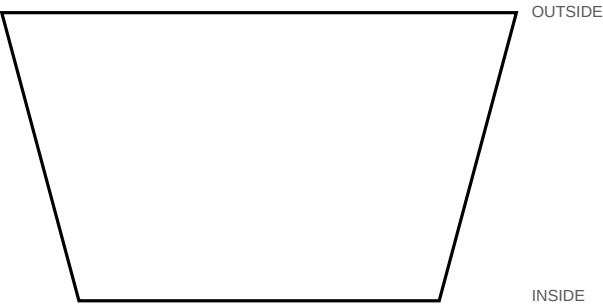
S3 · Ring 3 · make 12 12 segments · miter 15° each end Outside 2.679" · Inside 1.876" · Width 1.500" Stock thickness 0.750"
