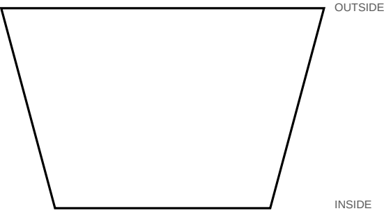
S2 · Ring 2 · make 12 12 segments · miter 15° each end Outside 2.412" · Inside 1.608" · Width 1.500" Stock thickness 0.750"
