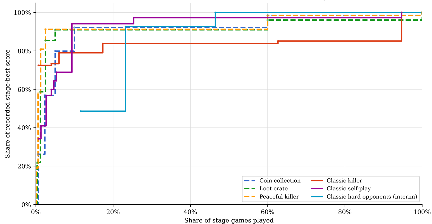
Normalized best-score improvement within each stage
