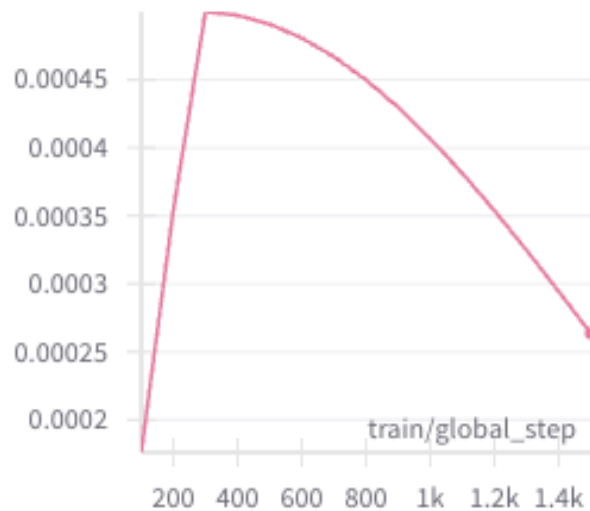
train/learning_rate
