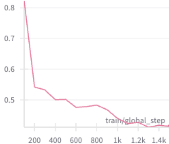
train/loss
