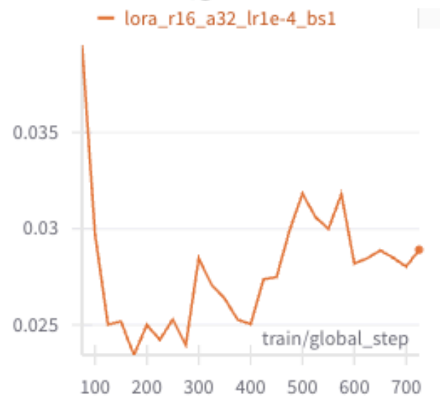
train/grad_norm
