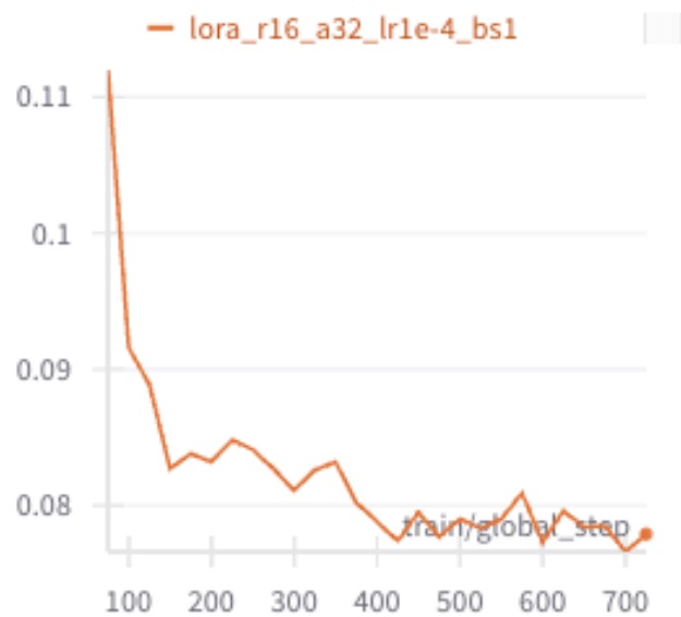
train/loss
