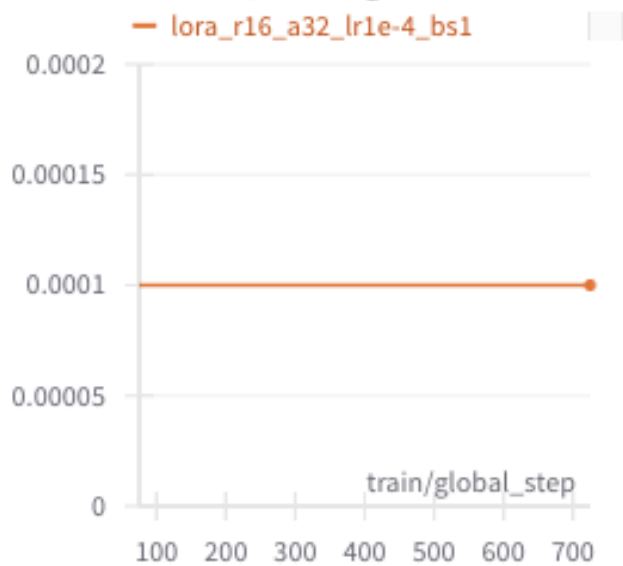
train/learning_rate
