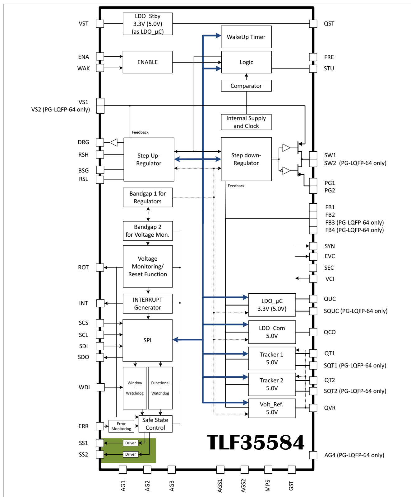
Figure 1 Block Diagram
