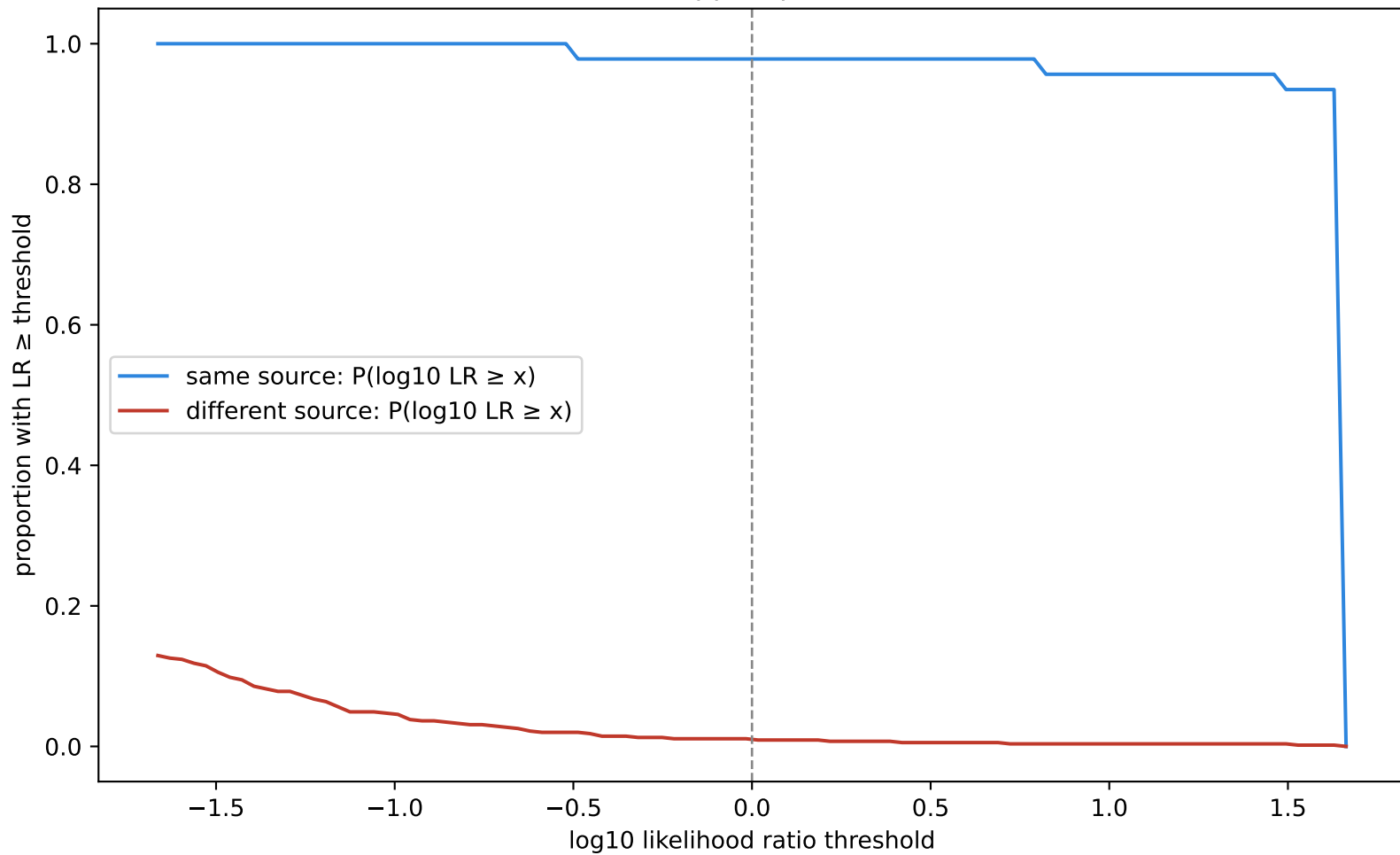
Tippett plot
