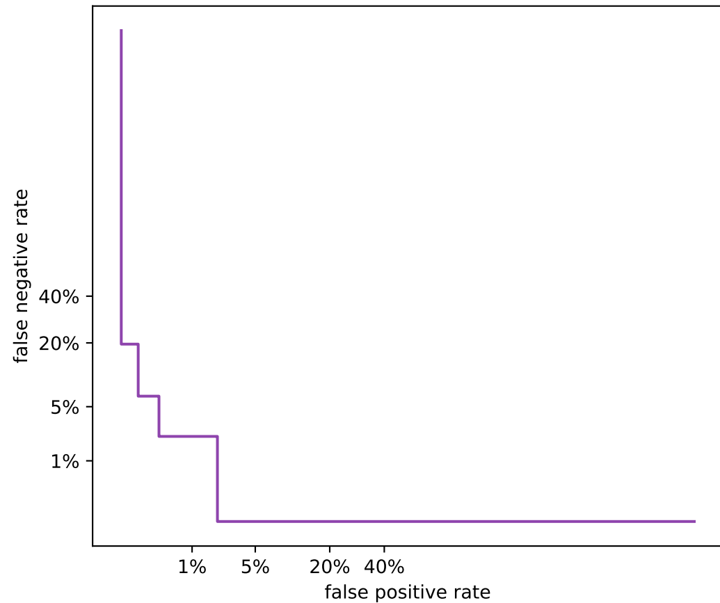
DET (EER = 2.1%)
