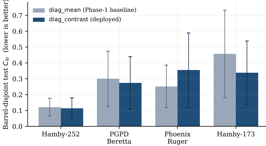
Figure 1. Barrel-disjoint test C_{lr} per study, baseline (diag_mean) vs deployed (diag_contrast); error bars are the cross-fold standard deviation. Generated from data/ablation.json . The wide error bars on the smaller NBTRD sets are the honest signature of limited source-disjoint data.
