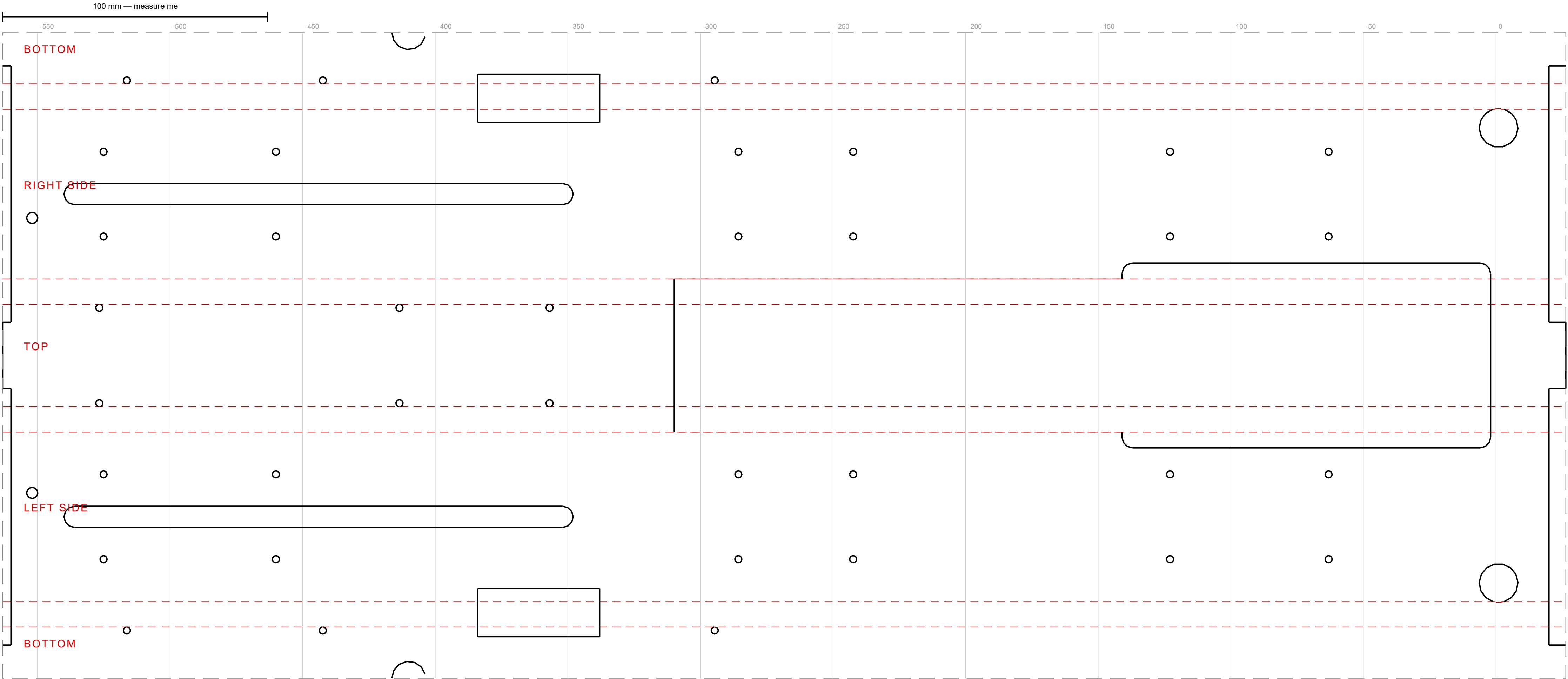
M2 core tube — 2x3x0.120 wall. Wrap 1:1. Seam on TOP centreline. Red dashed = corner tangents (fold lines), NOT cuts. Ticks are X in mm from the model origin. Tube length 589.52 mm, wrap 243.53 mm. Breech at left, muzzle at right.
