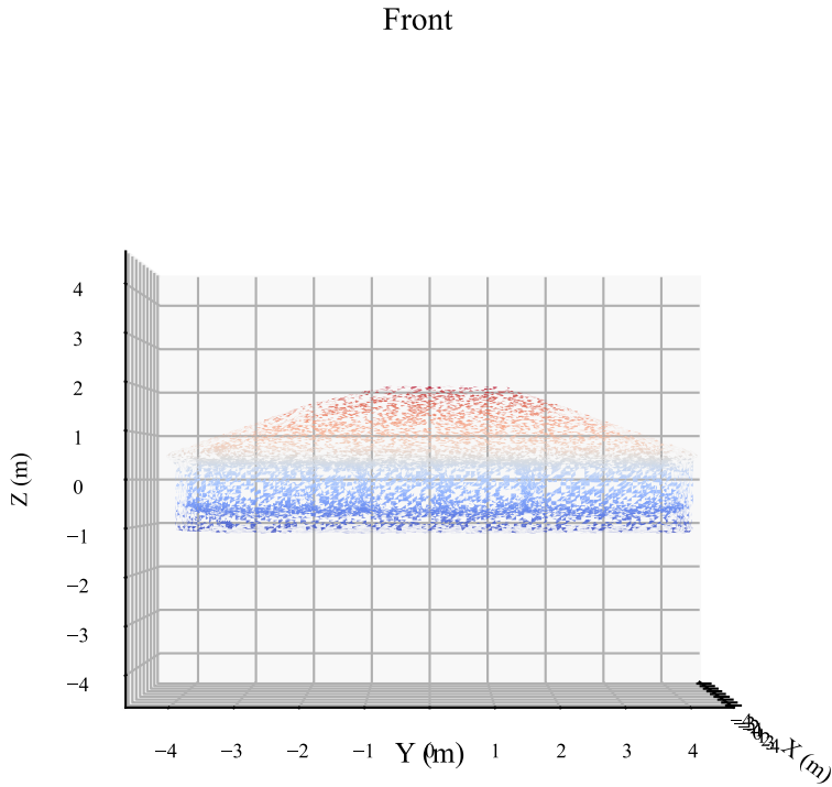
(b) Optimized V11 (64,280 voxels, -45.0%)
