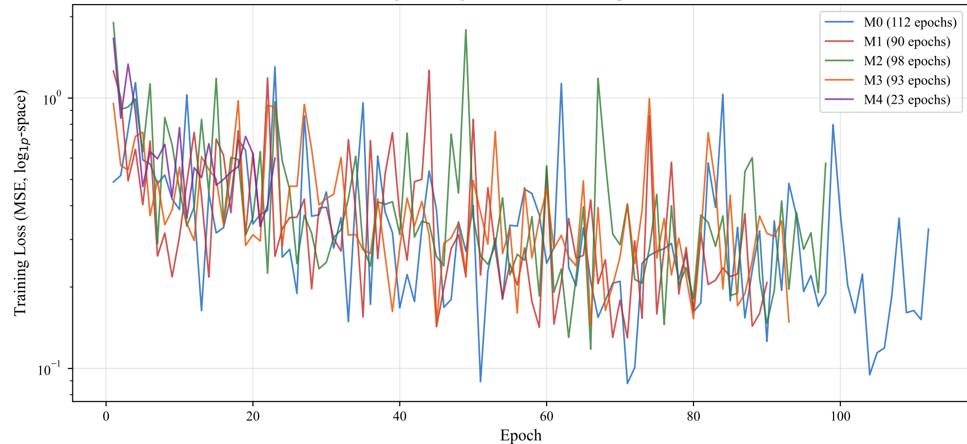
Training Convergence: 5-Member Deep Ensemble
