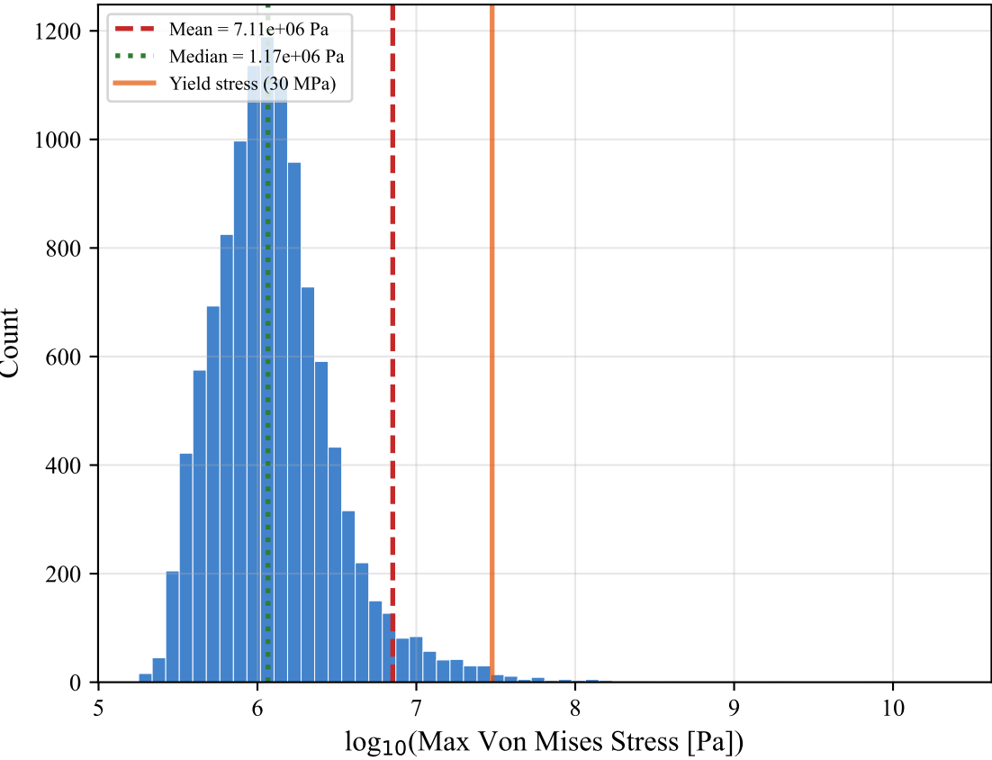
(a) Von Mises Stress Distribution
