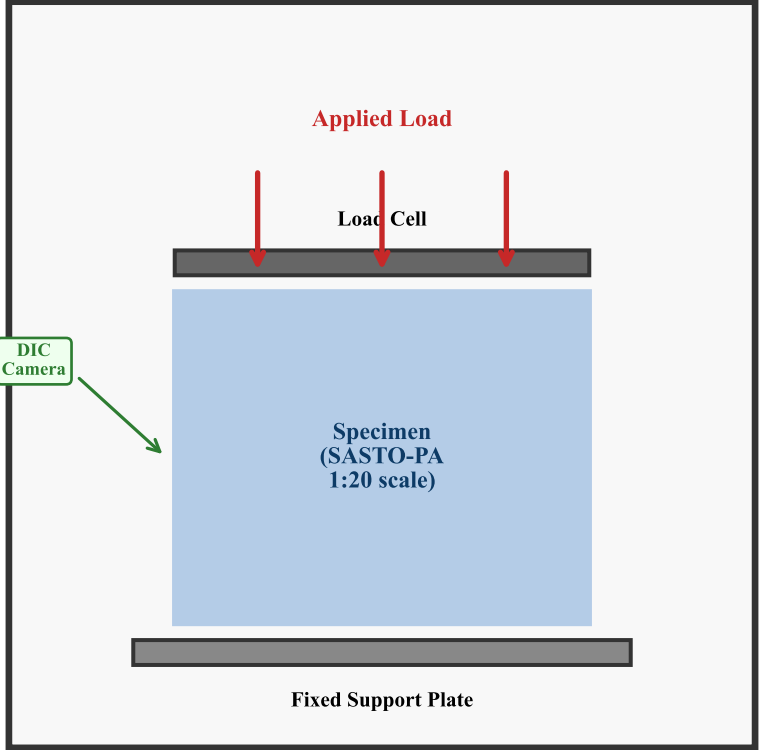
(b) Compression Test Setup (ASTM C39 adapted)
