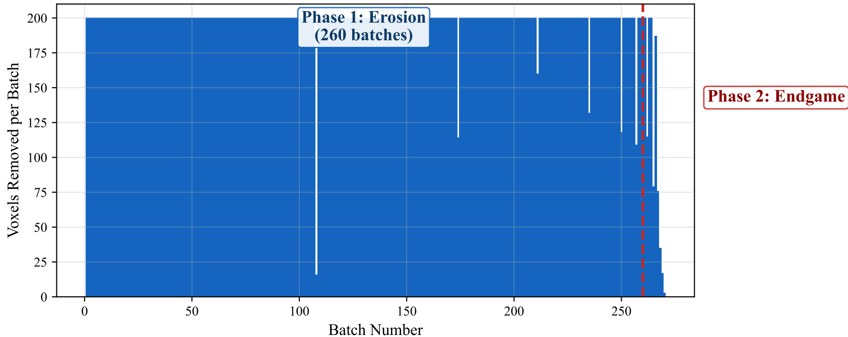
Adaptive Batch Size During SASTO-PA Optimization
