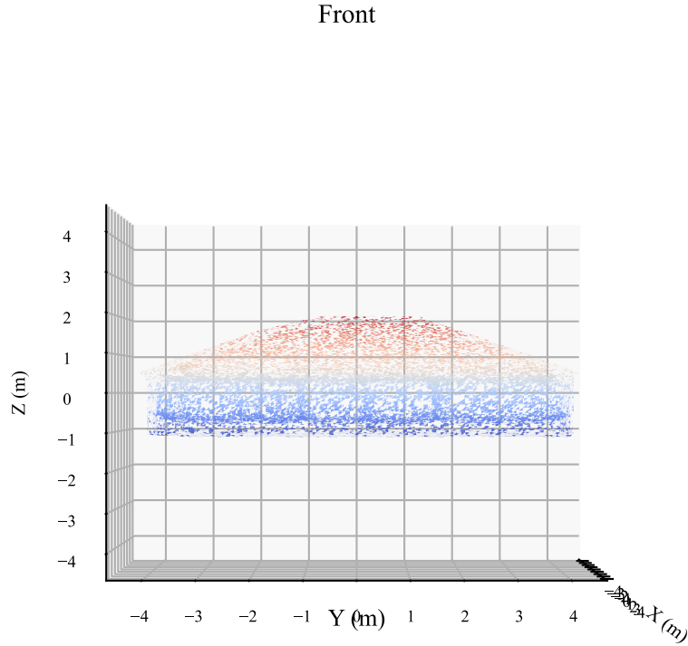
(b) Optimized SASTO-PA (64,280 voxels, -45.0%)
