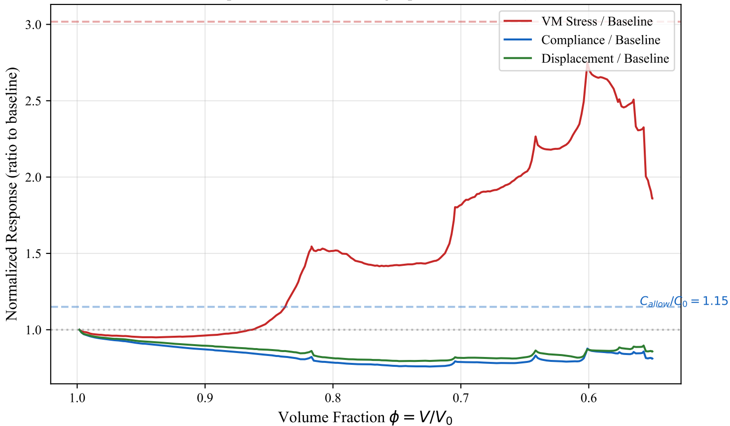
Response Evolution During Optimization (V11)
