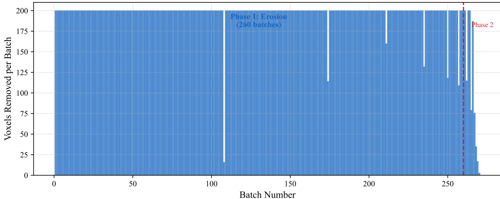
Adaptive Batch Size During V11 Optimization
