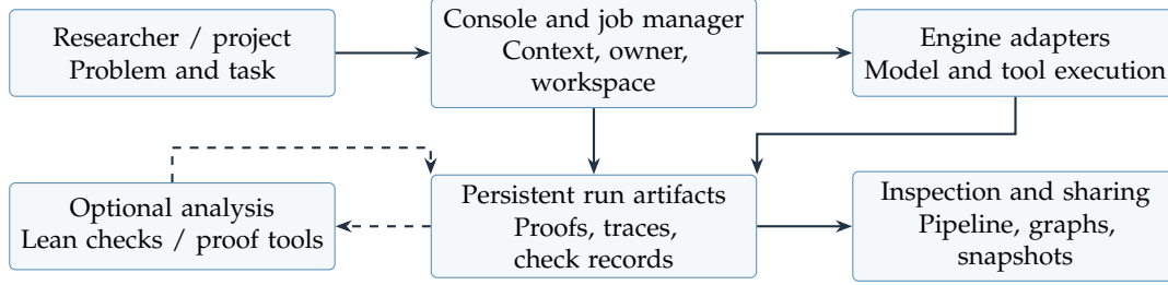
Figure 1: Main components and evidence flow. Dashed connections indicate optional analysis. Execution traces and proof dependencies are distinct artifacts.
