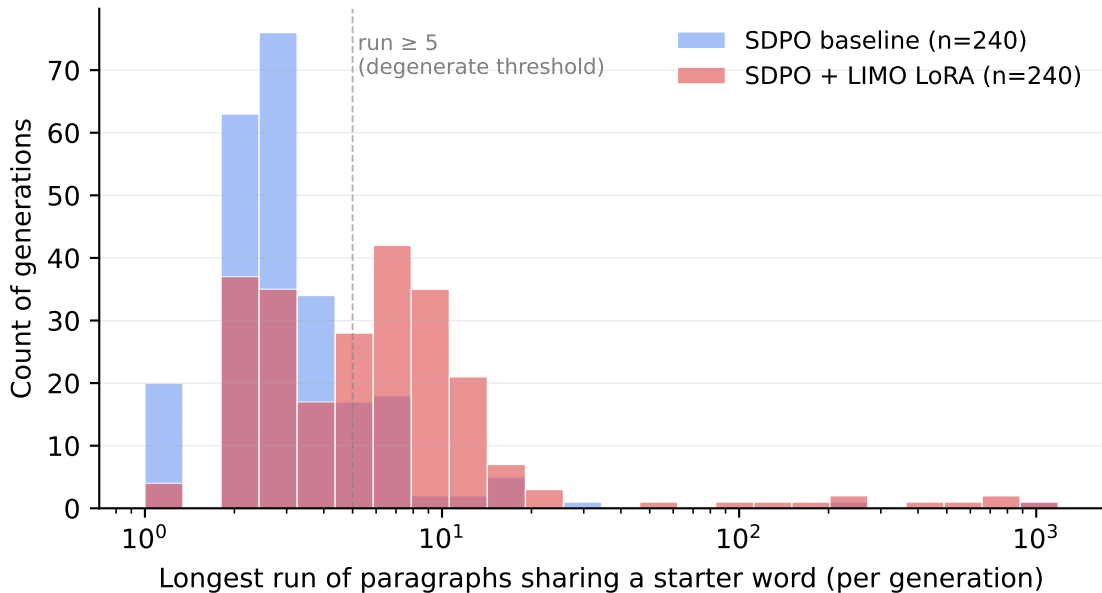
Off-policy LIMO LoRA induces a heavy tail of structural repetition
