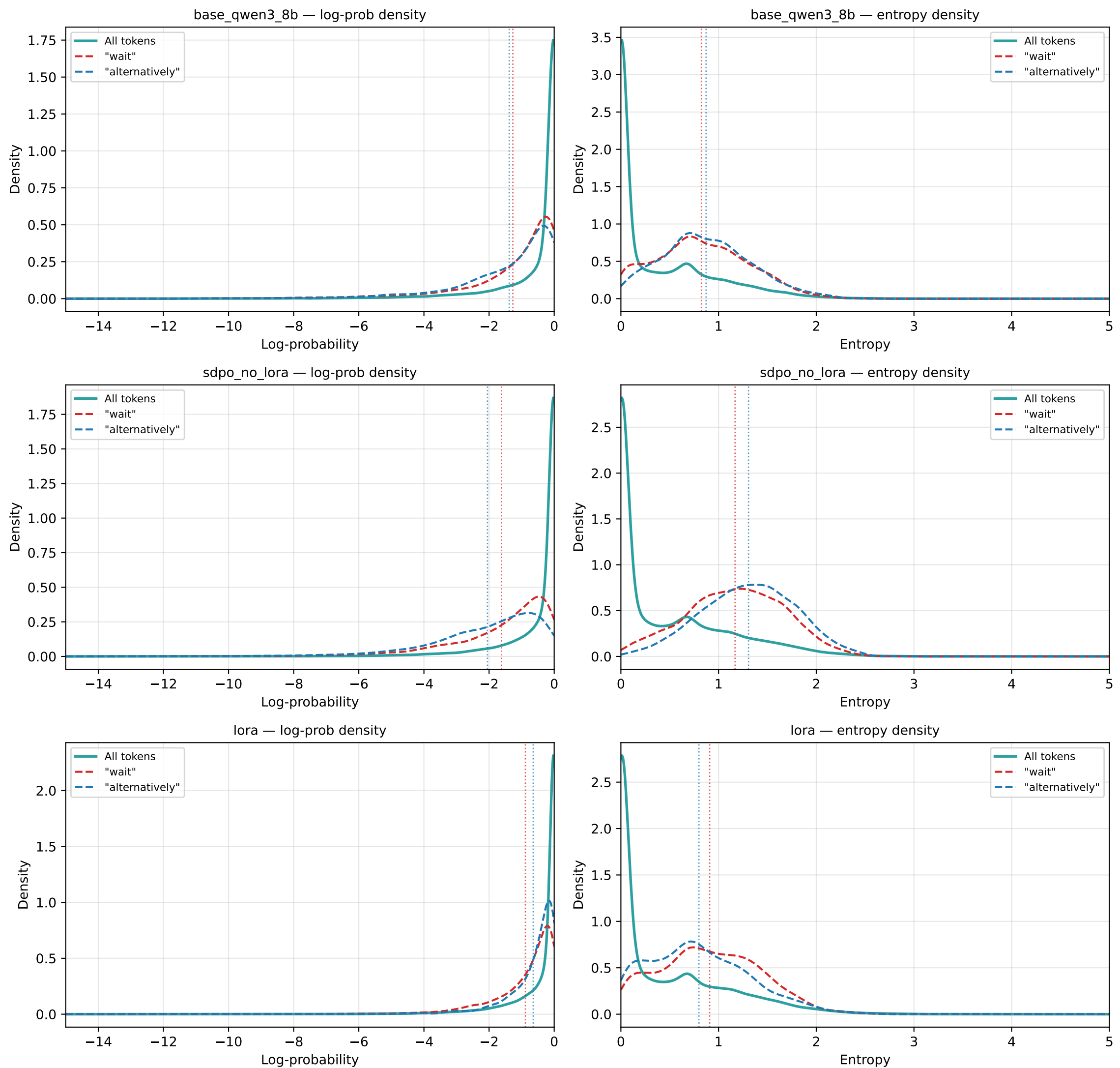
Figure 9 — log-prob & entropy density per model (teal: all tokens | red dashed: "wait" | blue dashed: "alternatively")
