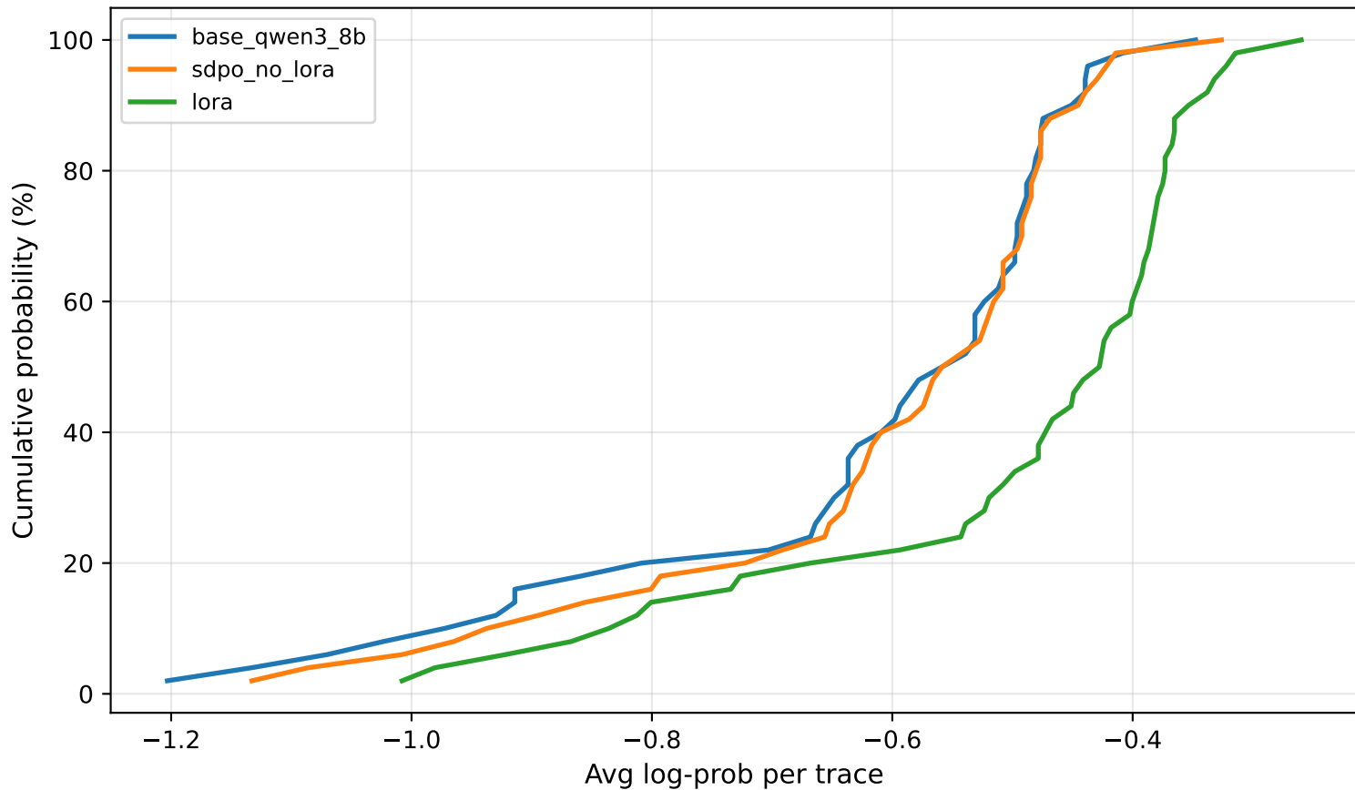
CDF of per-trace mean log-probability
