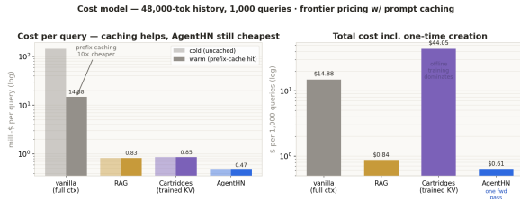
Figure 4: Cost per query and total cost over 1,000 queries against a 48k-token history, at representative frontier API pricing with prompt caching. scripts/cost_model.py .
