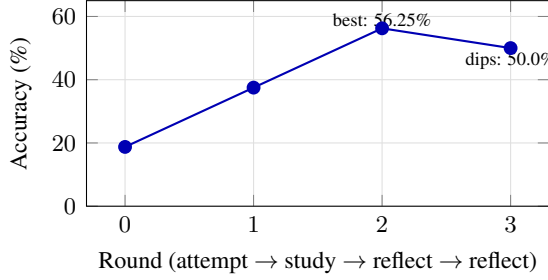
Figure 6: Self-improvement accuracy trajectory, real numbers, no keep-best ratchet: 18.75% → 37.5% → 56.25% → 50.0%. At every round, the test prompt contains only the bare question. src/agenthn/webapp/skills_service_product.py .
