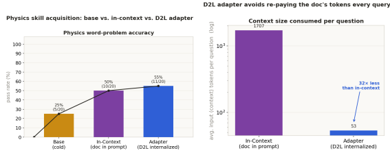
Figure 5: Physics word-problem accuracy (left) and query-time context (right): base vs. in-context vs. D2L adapter, on 20 held-out problems. skill-acquisition/make_physics_charts.py .
