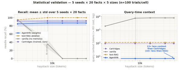
Figure 3: Statistical validation: 5 seeds \times 20 facts \times 5 sizes ( n=100 /cell), mean \pm std, Wilson 95% CIs. scripts/large_scale_eval.py.
