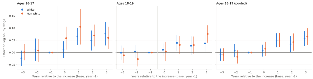
Teen wages by race (non-Hispanic white vs all other), 95% intervals
