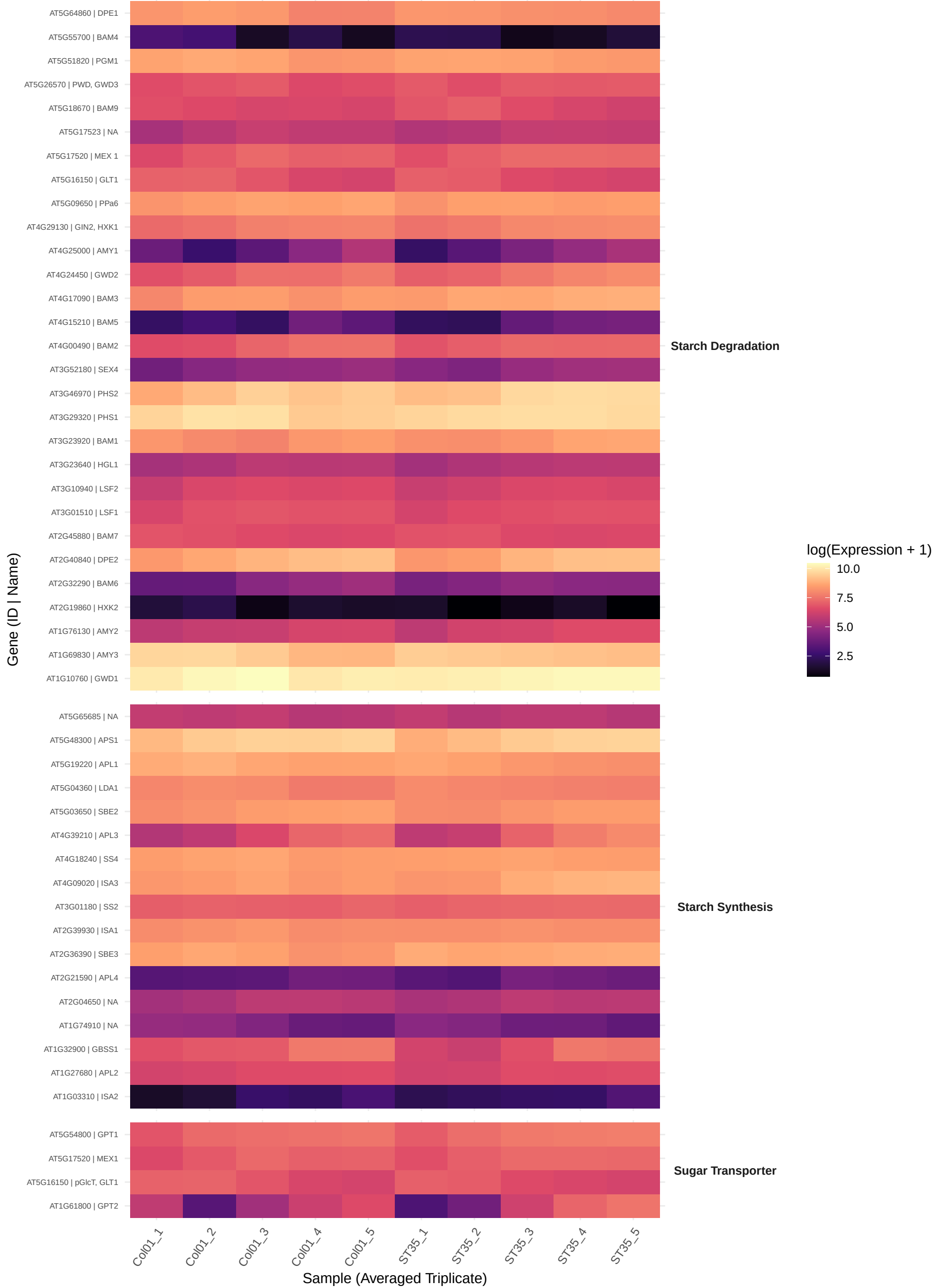
Starch Biosynthesis Gene Expression Heatmap
