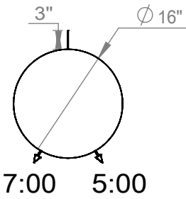
SECTION C-C 33-36 (A)
