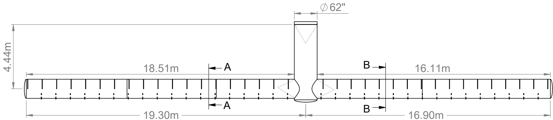
Vista Frontal
