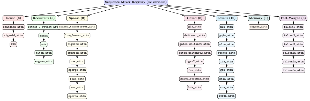
Figure 2: Comprehensive taxonomy of forty-two sequence mixer variants across seven functional categories. Dense baselines provide full global routing at quadratic cost. Recurrent architectures enable constant-time inference through state compression. Sparse variants reduce complexity through structured patterns or token selection. Gated mechanisms introduce data-dependent control over memory retention and forgetting. Latent methods compress key-value representations into low-rank bottlenecks or route through probabilistic Gaussian-mixture latents. Conditional memory provides test-time read/write over an external memory bank. Fast-weight methods treat the recurrent state transition as an online continual-learning rule.
