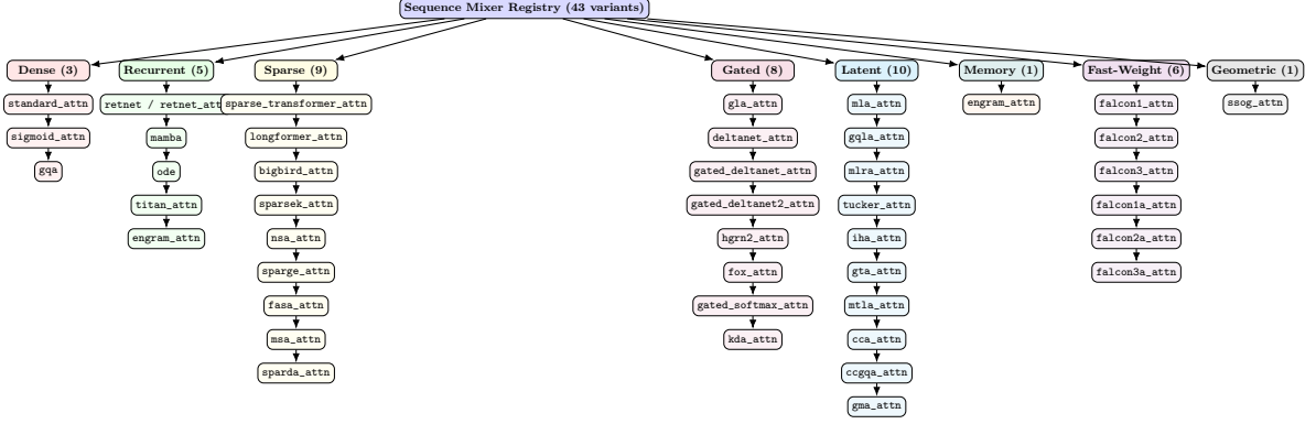
Figure 2: Comprehensive taxonomy of forty-three sequence mixer variants across eight functional categories. Dense baselines provide full global routing at quadratic cost. Recurrent architectures enable constant-time inference through state compression. Sparse variants reduce complexity through structured patterns or token selection. Gated mechanisms introduce data-dependent control over memory retention and forgetting. Latent methods compress key-value representations into low-rank bottlenecks or route through probabilistic Gaussian-mixture latents. Conditional memory provides test-time read/write over an external memory bank. Fast-weight methods treat the recurrent state transition as an online continual-learning rule. Geometric-field methods encode spatial or graph-structured inductive biases over the attention matrix.
