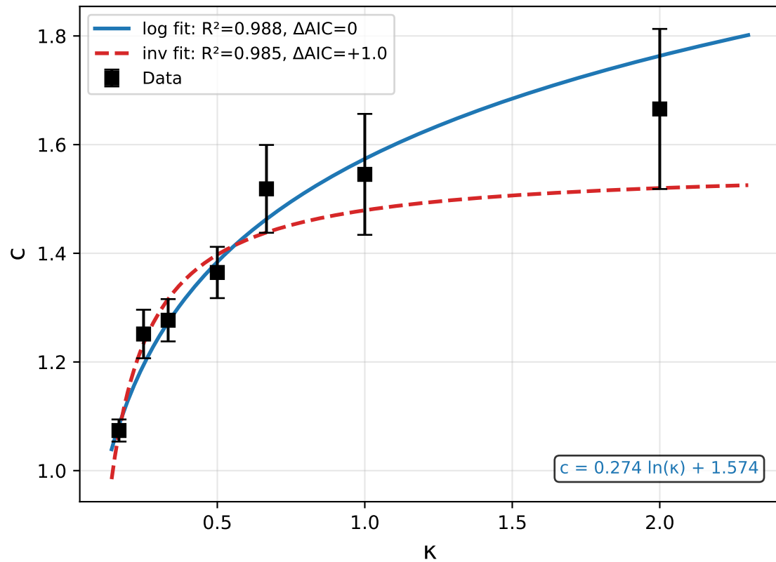
Bose-Hubbard sonic horizon (7 values of \kappa )
