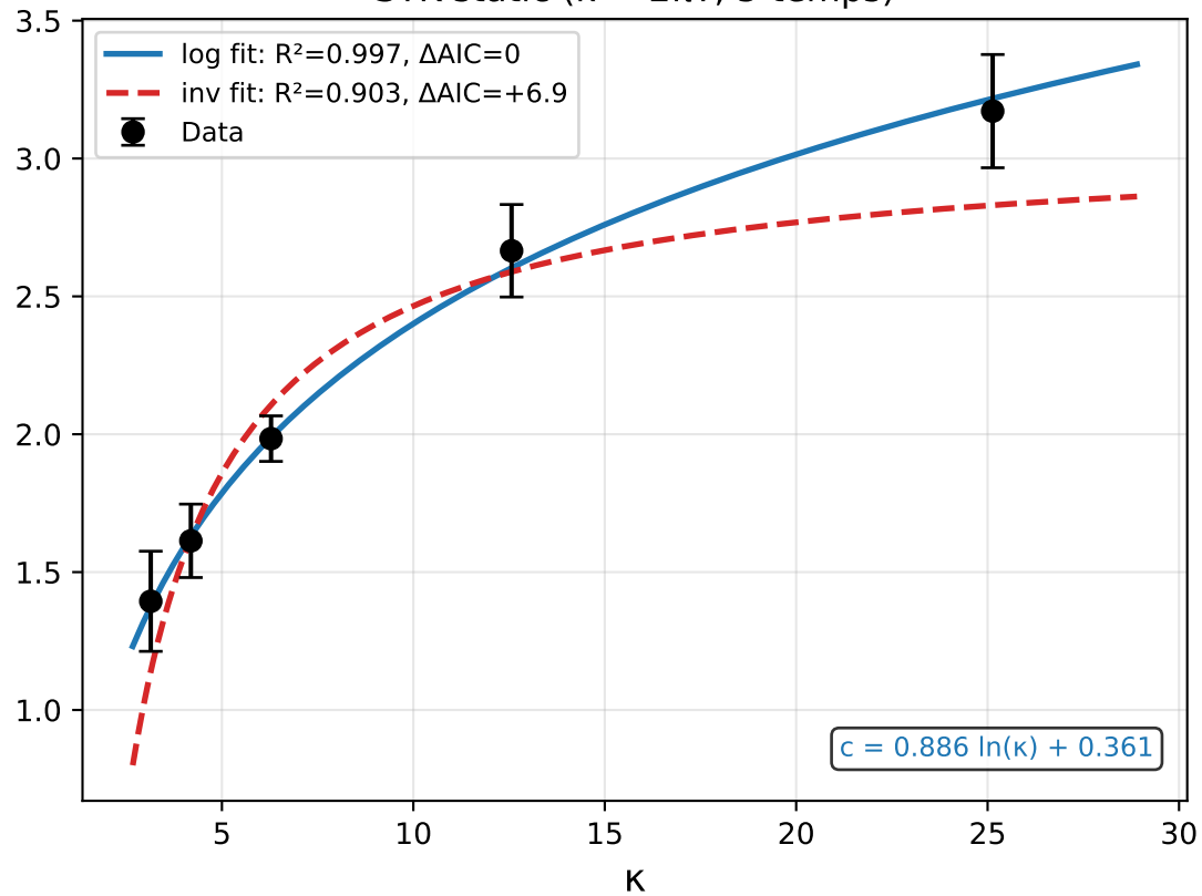
SYK static ( \kappa = 2\pi T , 5 temps)
