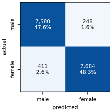
(b) CharTransformer
