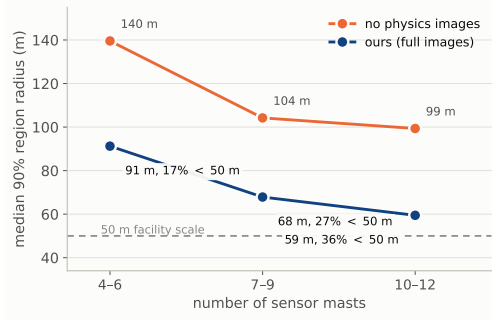
Fig. 3. Sensor-count ablation (measured wind, seed-1 diagnostic; prespecified bands of n=690/635/675 scenarios). More masts shrink the guaranteed regions and raise the share at the facility scale; the conformal guarantee remains marginal over the full distribution.
