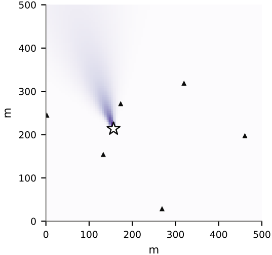
CH4 plume: 367 kg/h, 4.6 m/s, class B
