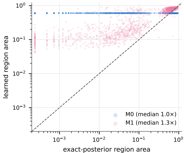
CH4-500: sharpness at matched 90% coverage
