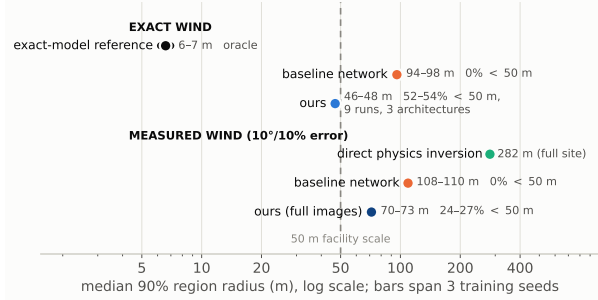
Fig. 3. The study in one view: median 90% region radius by method and wind condition (log scale; bars span 3 training seeds; fractions below the 50 m facility scale annotated). Physics images halve the exact-wind regions; under measured wind, direct inversion returns the full site while the learned recipe holds 70–73 m.
