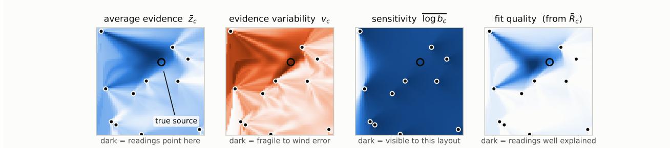
Fig. 7. The four physics input images for one test scenario (closed form, computed from the network's own inputs at the measured wind): average evidence, evidence variability across the wind-error range, sensitivity, and fit quality. The circle marks the true source; dots mark the sensor masts.
