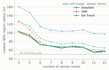
Fig. 3. Sensor-count ablation for all three base networks (measured wind, seed-1 diagnostic; \approx 210 – 240 test scenarios per mast count; solid: with images, dashed: without). With the images, the three networks track a single curve that approaches the facility scale as masts are added; the conformal guarantee remains marginal over the full distribution.
