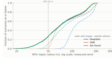
Fig. 4. Region-radius distributions over all 2,000 test scenarios under measured wind, for all three base networks (seed 1; solid: with images, dashed: without). The three with-images distributions are nearly indistinguishable: the physics images, not the architecture, set the achievable precision; about a quarter of regions fall below the 50 m scale.
