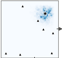
DeepSets localizer (posterior heatmap)
