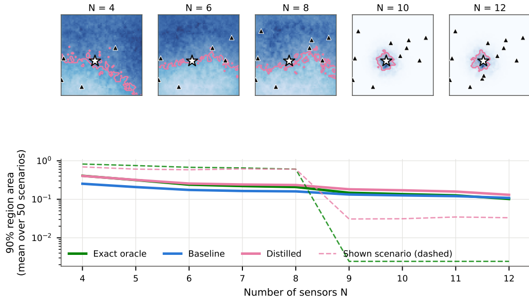
Figure 3: Dose-response flagship. Top: one base scenario as sensors accrue 4 \rightarrow 12 (physics-distilled heatmap; region as translucent fill; star = true source). Bottom: mean region area vs. N for the exact oracle, baseline, and distilled model (dashed: the shown scenario).
