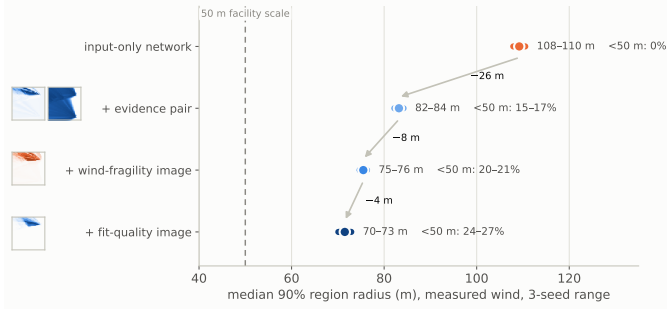
Fig. 3. Each physics image, added on top of the input-only network, tightens the guaranteed regions (DeepSets base, measured wind; 3-seed ranges; the map added at each step is shown beside its row).
