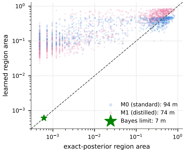
CH4-T: sharpness at matched 90% coverage
