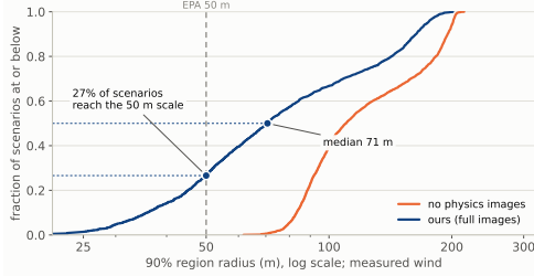
Fig. 4. Region-radius distributions over all 2,000 test scenarios under measured wind. The annotated points show how the headline statistics coexist: 27% of scenarios fall below the 50 m facility scale while the median sits at 71 m; the no-images distribution never reaches the scale.
