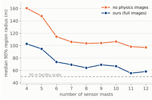
Fig. 3. Sensor-count ablation (measured wind, seed-1 diagnostic; \approx 210 – 240 test scenarios per mast count). More masts shrink the guaranteed regions toward the facility scale; the conformal guarantee remains marginal over the full distribution.
