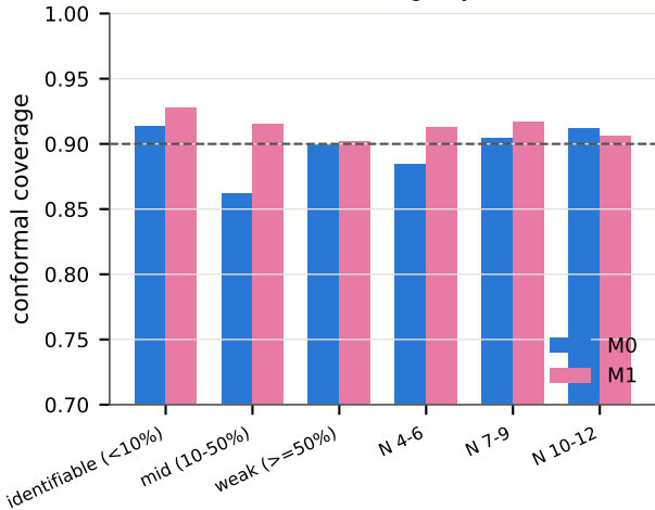
Conditional coverage by stratum
