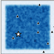
Amortized heatmap
