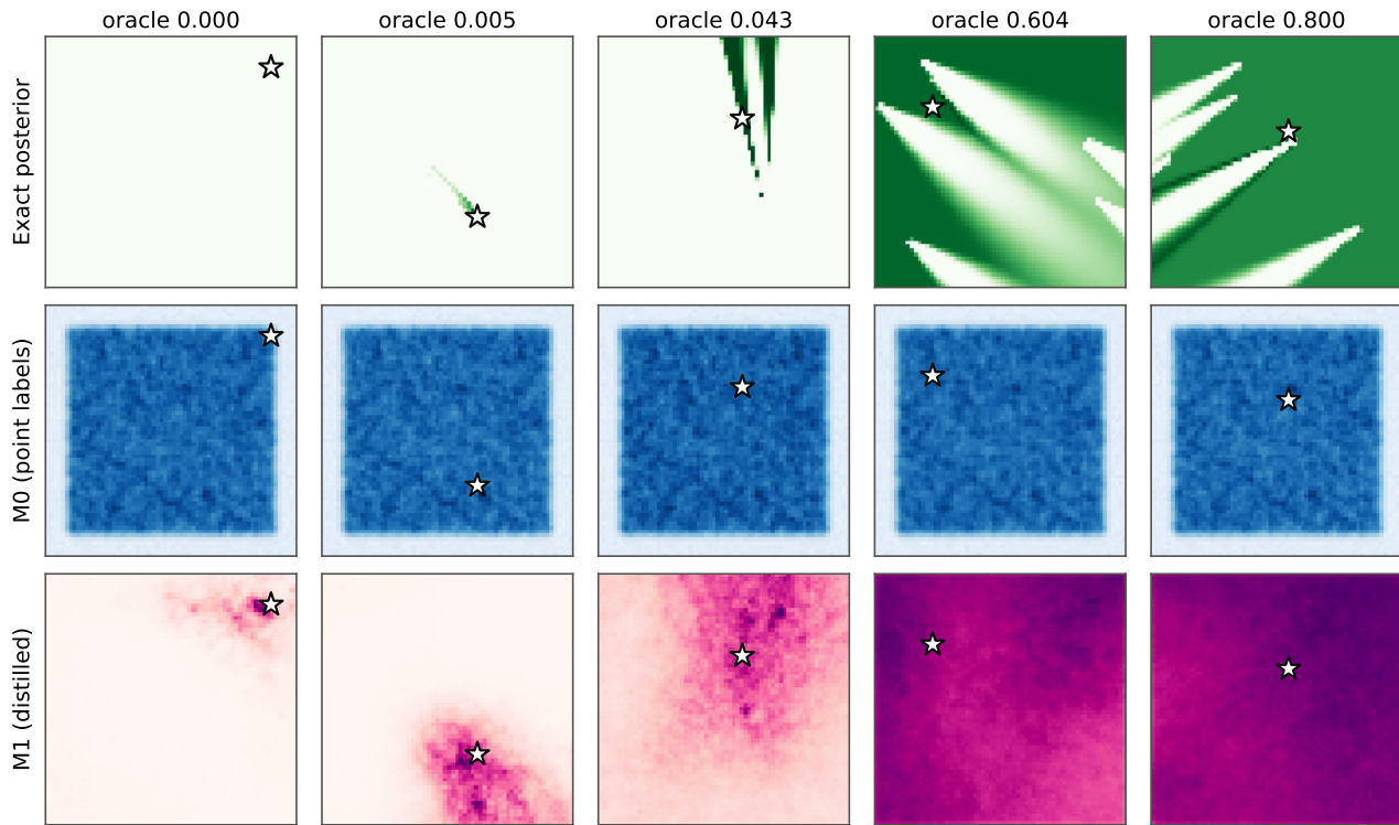
Posterior shape across identifiability
