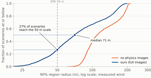
Fig. 3. Region-radius distributions over all 2,000 test scenarios under measured wind. The annotated points show how the headline statistics coexist: 27% of scenarios fall below the 50 m facility scale while the median sits at 71 m; the no-images distribution never reaches the scale.
