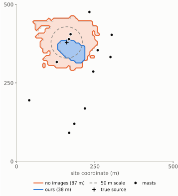
Fig. 1. A well-instrumented test scenario (12 masts, measured wind): 90% regions of the no-images baseline and of our method (conformal masks), with the 50 m facility scale. Selection rule: among scenarios with \geq 10 masts whose region meets the 50 m scale, the one at that subset’s median radius, i.e., representative of the quarter of cases that reach the scale (Fig. 3), not a best case.
