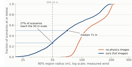
Fig. 4. Region-radius distributions over all 2,000 test scenarios under measured wind: 27% of our regions fall below the 50 m scale while the median sits at 71 m; the no-images distribution never reaches the scale.
