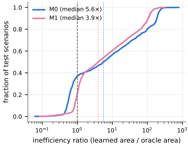
Inefficiency distribution
