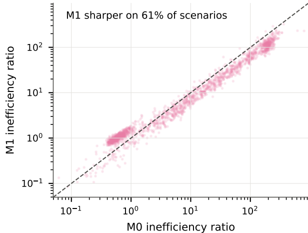
Per-scenario improvement
