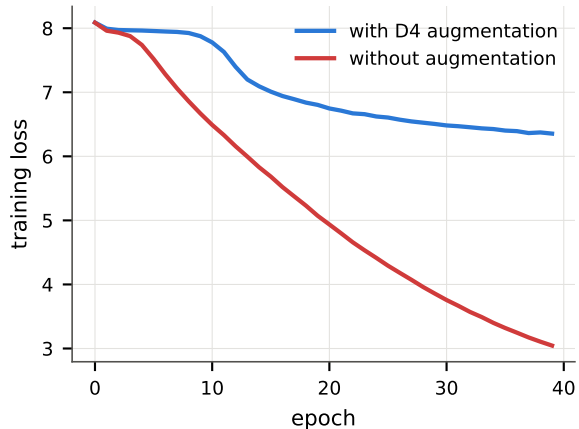
Memorization without symmetry augmentation
