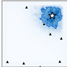
90% conformal region
