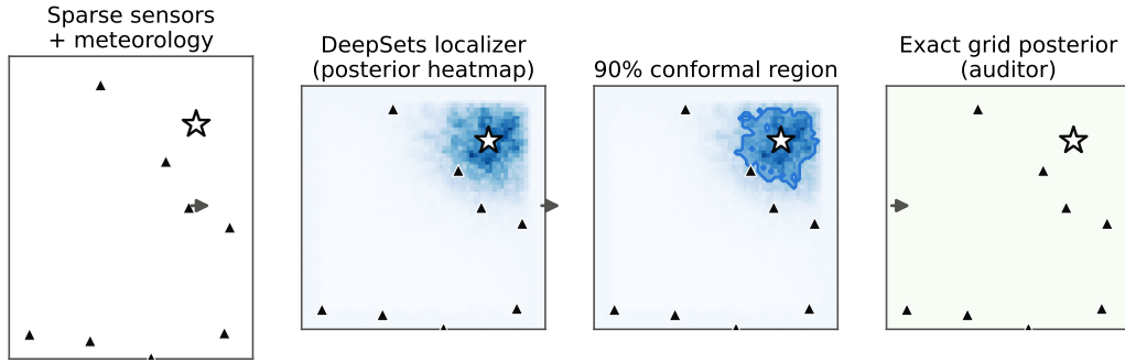
Figure 11: Pipeline on a real median-difficulty test scenario (M0; star = true source, triangles = sensors): readings \rightarrow amortized heatmap \rightarrow 90% conformal region; the exact grid posterior is teacher (train/val) and reference (calib/test).
