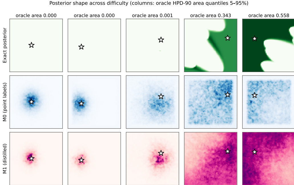
Figure 3: Posterior shape across difficulty. Columns: five test scenarios at oracle HPD-90 area quantiles (5–95%). Rows: exact posterior, M0, M1 (same scenario per column; star = true source). Distillation transfers the oracle’s shape — sharp peaks, ridges, multimodality — that point labels cannot supervise.
