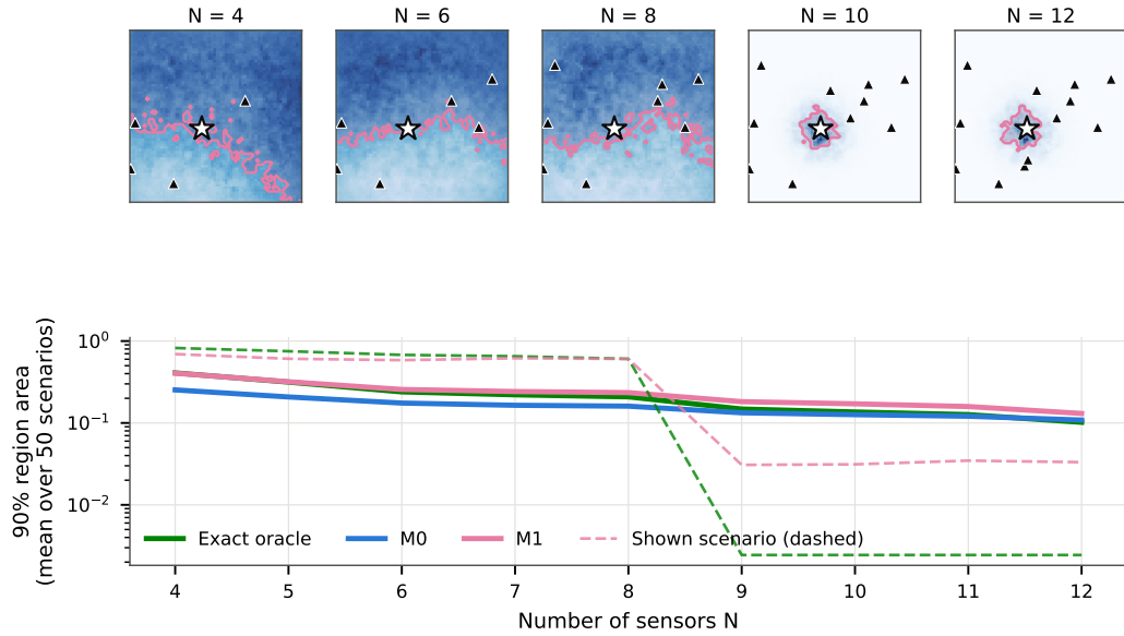
Figure 5: Information dose-response. Top: one base scenario as sensors accrue 4 \rightarrow 12 (best model’s heatmap; region as translucent fill; star = true source). Bottom: mean 90% region area vs. N for the exact oracle, M0, and M1.
