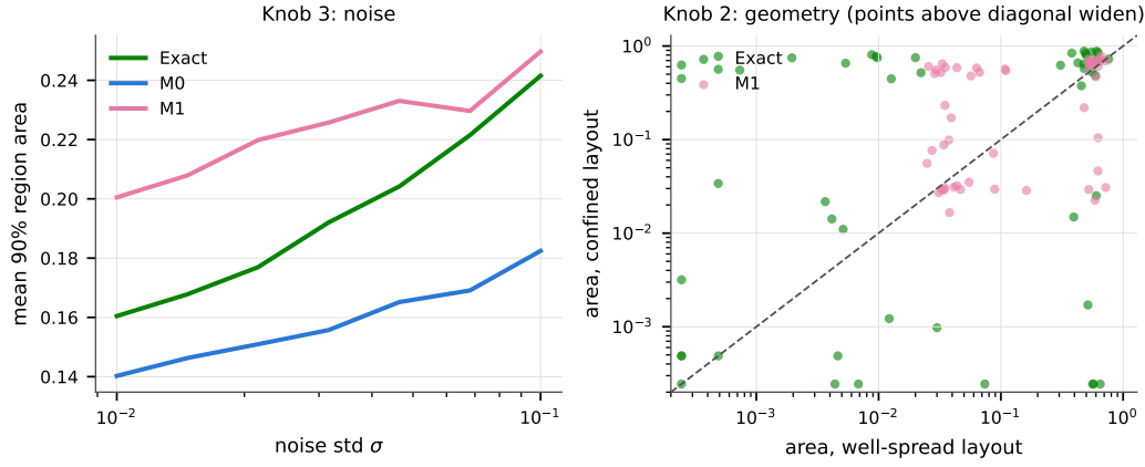
Figure 10: Remaining dose-response knobs. Left: mean region area under the noise sweep (Knob 3). Right: matched geometry pairs (Knob 2); points above the diagonal widen under the confined layout, as the physics dictates.
