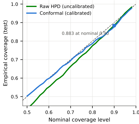
Figure 2: Coverage vs. nominal (M0) . Conformal regions track the diagonal; raw HPD undercovers. Coverage is thereby equalized across models, making region size a pure sharpness measurement.
