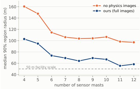
Fig. 3. Sensor-count ablation (measured wind, seed-1 diagnostic; \approx 210 –240 test scenarios per mast count). More masts shrink the guaranteed regions toward the facility scale; the conformal guarantee remains marginal over the full distribution.
