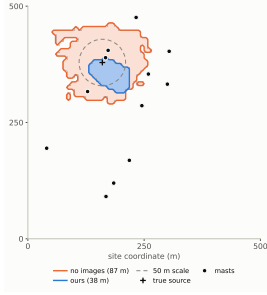
Fig. 1. A well-instrumented test scenario (12 masts, measured wind): 90% regions of the no-images baseline and of our method (conformal masks), with the 50 m facility scale. Selection rule: among \geq 10 -mast scenarios whose region meets the 50 m scale, the one at that subset’s median radius: representative of the quarter of cases that reach the scale (Fig. 4), not a best case.
